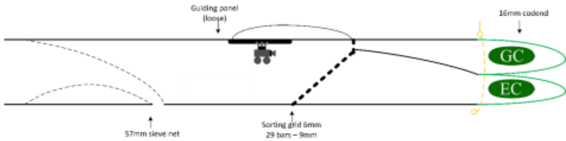
Figure 10: Details of design SG2. The green ellipses represent the two experimental compartments considered.
