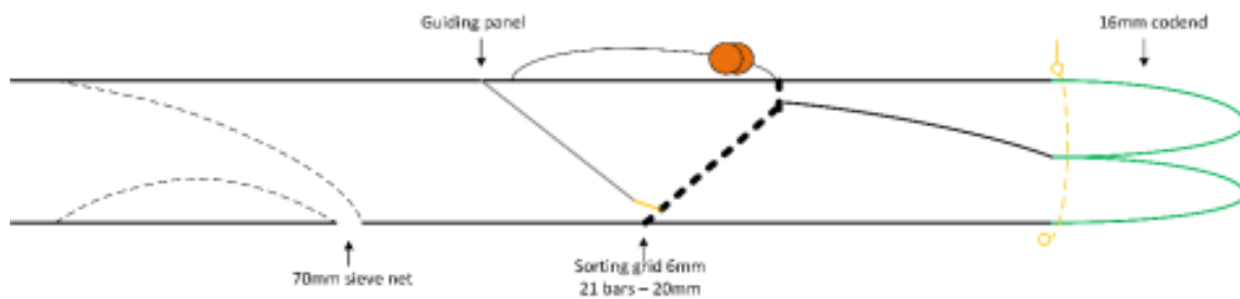
Figure 9: Details of Single-grid gear Design 1
