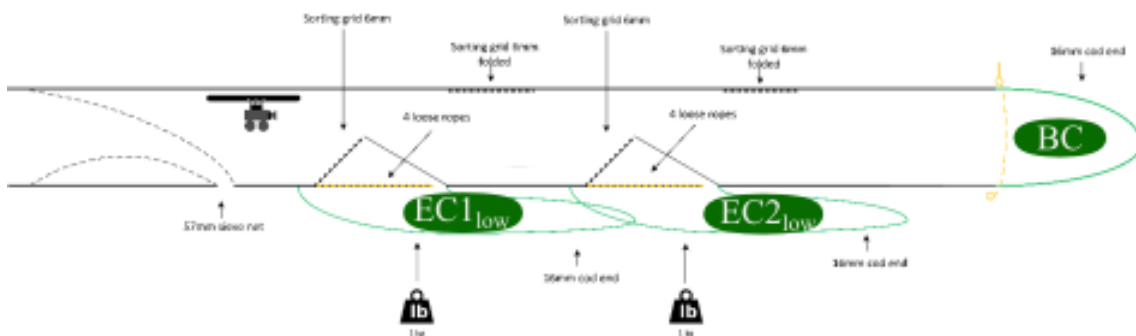
Figure 19: Details of Multi-grid gear design MG5
