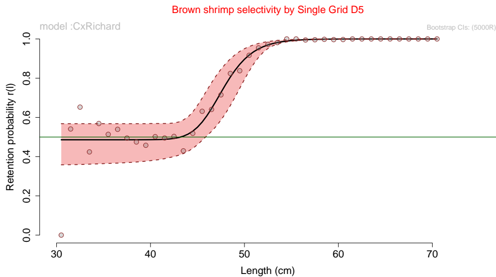
Figure 20: Average sorting efficiency curve and 95% bootstrap CL's estimated for design SG5 by the best candidate model. Points represent the proportion of catch of length l estimated in the GC.
