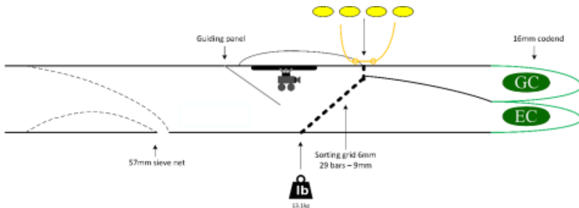
Figure 13: Details of design SG5
