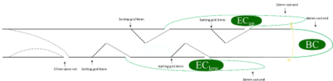
Figure 16: Details of Multi-grid gear design MG2
