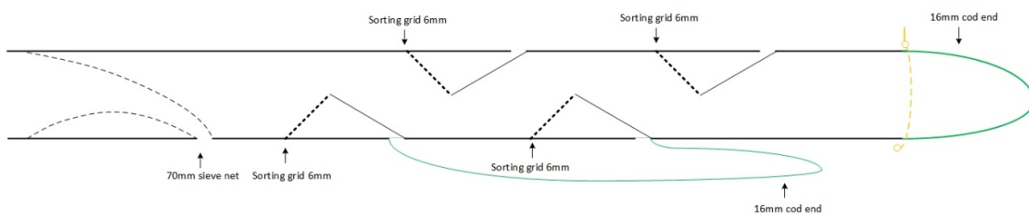
Figure 3: Side view of the Multi-grid gear.
