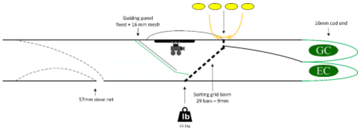
Figure 14: Details of design SG6
