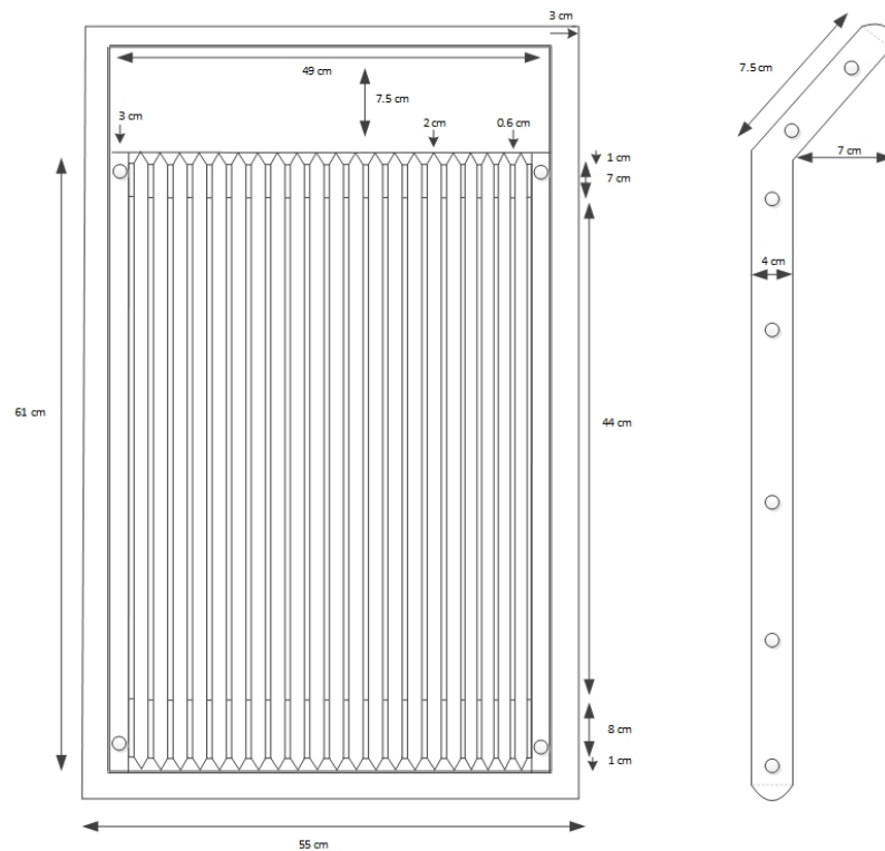
Figure 1: Constructive details of the single grid
