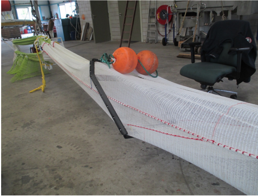
Figure 2: Single-grid gear under construction in the net loft. The oblique red selvedge is the connection of the guiding panel to the net tunnel.
