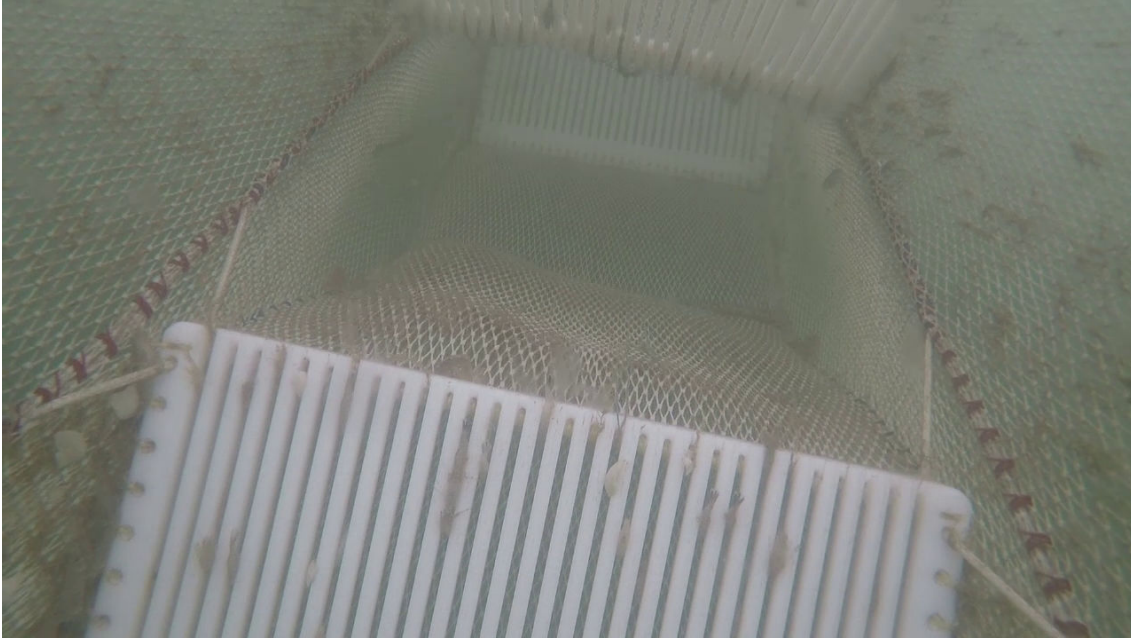
Figure 23: Top view of the front part of the multi-grid gear, showing the two upper grids and the front lower grid. The camera position can be checked in Figure 17
