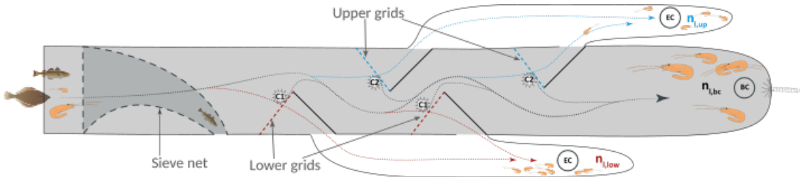
Figure 8: Expected transportation paths for brown shrimps entering in the grid zone, defining the catch share between the lower EC ( n_{l,low} ), upper EC ( n_{l,up} ) and BC ( n_{l,bc} )
