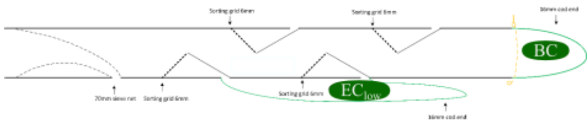
Figure 15: Details of Multi-grid design MG1
