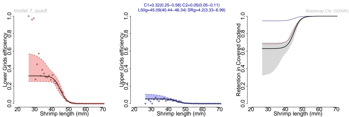
Figure 21: p_{low}(l) (left), p_{up}(l) (center) and global sorting efficiency (right) estimated for MG3 design
