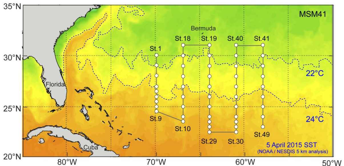
Figure 1. Map of the sampling stations of the MSM41 research cruise conducted in the Sargasso Sea in April 2015 showing the sea surface temperature (SST) patterns estimated for 5 April 2015 by the data-assimilative analysis of NOAA/Nesdis, which uses all available data for each day. The 22°C (northern front) and 24°C (southern front) are shown, since these temperature isotherms are associated with the locations where fronts can form in the Subtropical Convergence Zone of the Sargasso Sea during the autumn to spring seasons.
