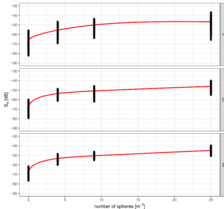
FIGURE 7: Predicted S_a values (solid line) and experimental values (black marks) depending on the number of spheres n per \text{m}^2 of netting, exemplarily at 130 kHz
