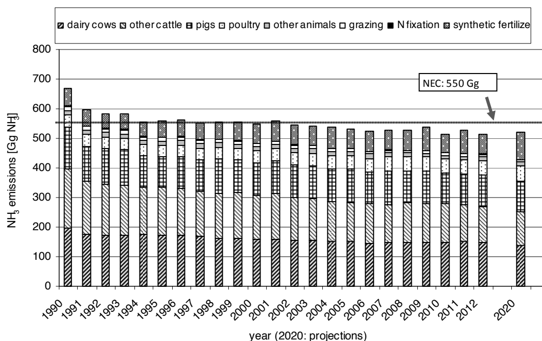
Figure 2.7: Annual \text{NH}_3 emissions from German agriculture and projections for 2020 (Submission 2014)
