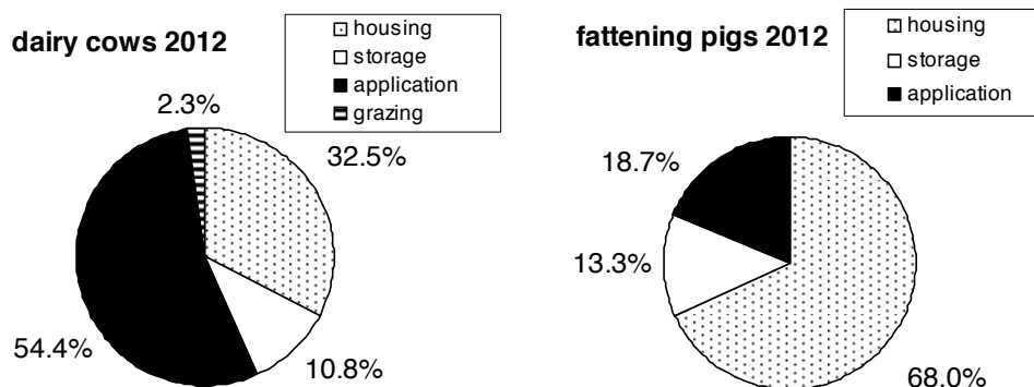
Figure 2.9: Dairy cows and fattening pigs (Submission 2014): Percentages of \text{NH}_3 emissions originating from housing, storage, manure application and grazing in 2012 (no free range husbandry for pigs)
