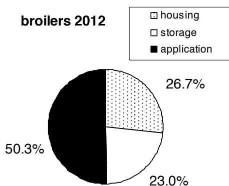
Figure 2.10: Broilers (Submission 2014): Percentages of \text{NH}_3 emissions originating from housing, storage, manure application and grazing in 2012
