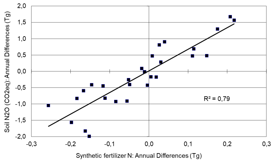
Figure 2.6: Interannual variations of annual N 2 O emissions (direct plus indirect N 2 O) from agricultural soils vs. interannual variations of mineral fertilizer N for the years 1990 to 2018 (Submission 2020)
