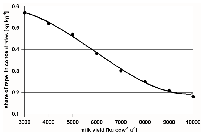
Figure 4.1: Standard mixed feeds, share of rapeseed expeller in concentrates (related to DM) as function of milk yield
