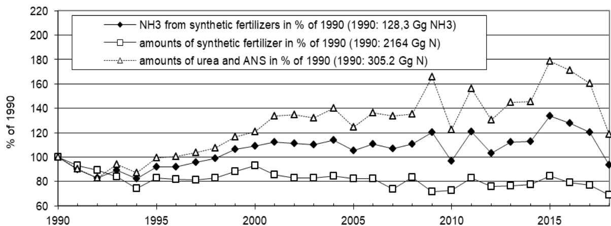
Figure 2.11: Application of mineral fertilizer N (amounts sold), amounts of N in urea and ANS applied, and the NH 3 emissions from the total application of mineral fertilizers (Submission 2020)
