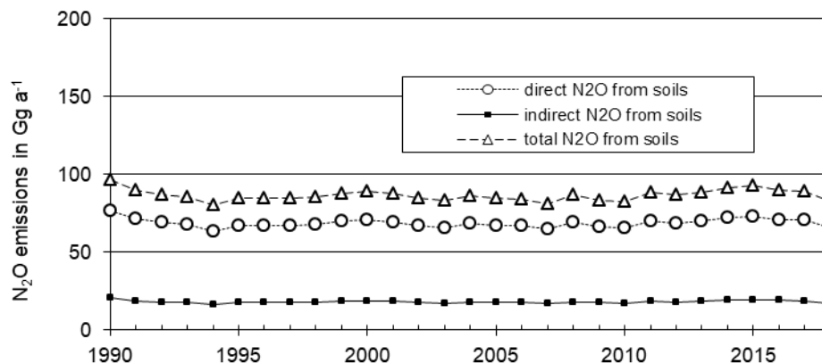
Figure 2.5: N 2 O emissions from agricultural soils (in Gg a -1 N 2 O), Submission 2020
