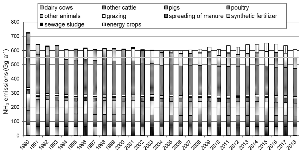
Figure 2.7: Annual NH 3 emissions from German agriculture for 1990 – 2018 (Submission 2020), National emission ceiling (NEC) at 550 Gg a -1
