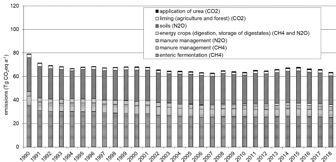
Figure 2.1: Annual THG emissions from German agriculture (Submission 2020) (GWP CH4 = 25, GWP N2O = 298)
