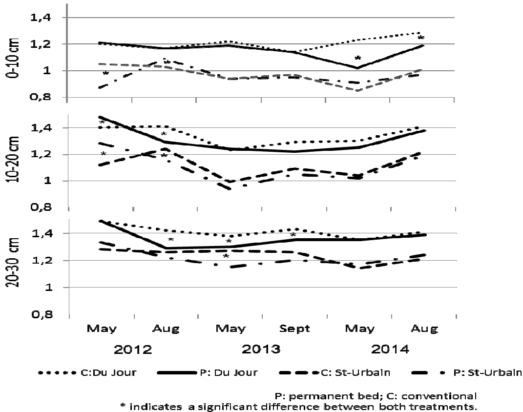
Figure 1. Evolution of soil bulk density over time
