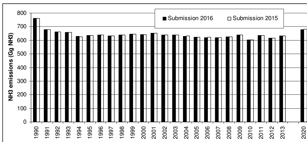
Figure 2.14: Comparison of \text{NH}_3 emission results in Submission 2016 and Submission 2015
