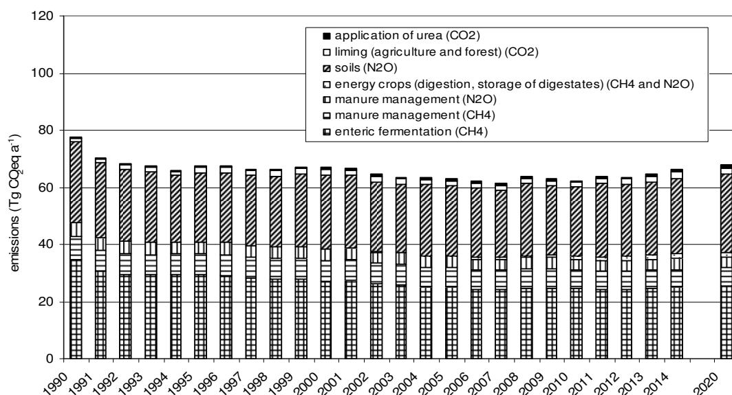
Figure 2.1: Annual THG emissions from German agriculture and projections for 2020 (Submission 2016) (GWP CH 4 = 25, GWP N 2 O = 298)
