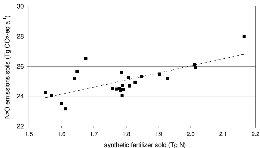
Figure 2.6: Total of annual N 2 O emissions (direct and indirect) from agricultural soils vs annual amounts of mineral fertilizer N for the years 1990 to 2014 (Submission 2016)
