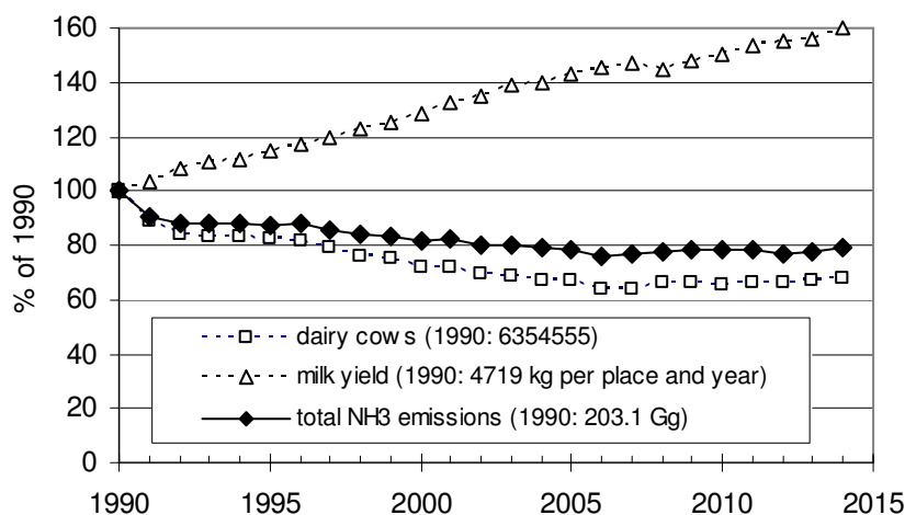
Figure 2.8: Development of dairy cattle numbers, milk yields and NH 3 from dairy cattle husbandry (including grazing), Submission 2016
