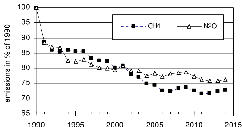
Figure 2.2: Development of CH 4 und N 2 O emissions from animal husbandry in % of 1990, Submission 2016 (enteric fermentation and manure management)
