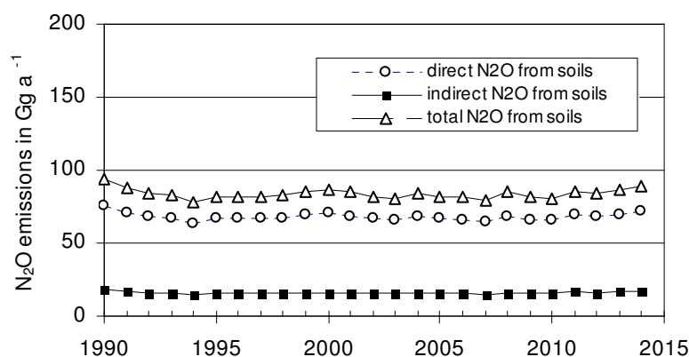
Figure 2.5: \text{N}_2\text{O} emissions from agricultural soils (in \text{Gg a}^{-1} \text{N}_2\text{O} ), Submission 2016
