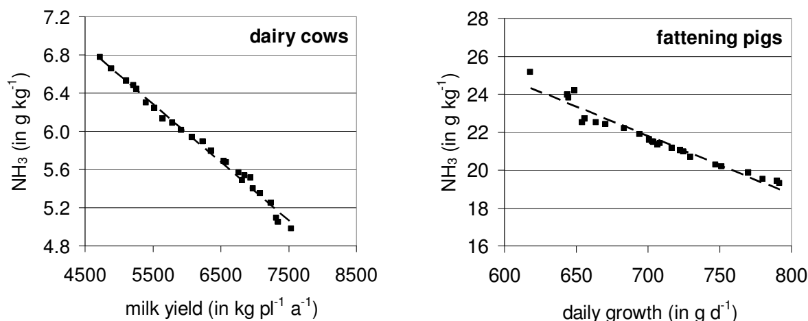
Figure 2.11: Dairy cows and fattening pigs: Performance-related total NH 3 emissions from animal husbandry, including grazing for dairy cows (for dairy cows per kg milk, for fattening pigs per g of daily growth), Submission 2016
