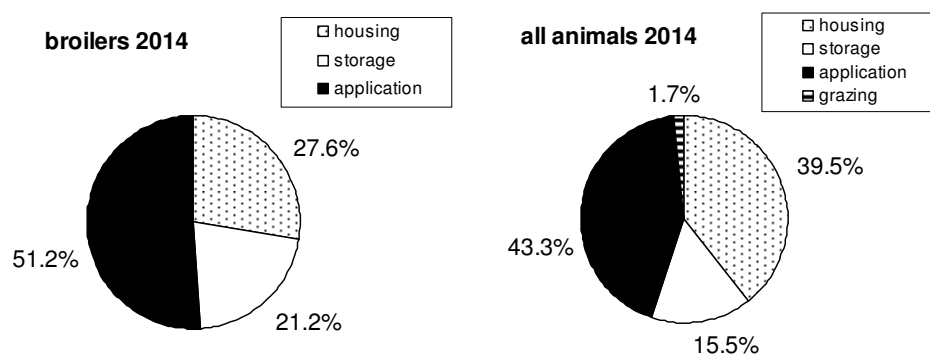
Figure 2.10: Broilers and all animals (Submission 2016): Percentages of NH 3 emissions originating from housing, storage, manure application and grazing in 2014
