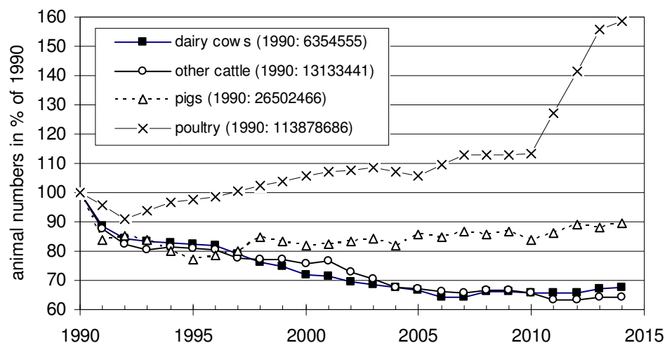
Figure 2.3: Development of animal numbers in % of 1990, Submission 2016
