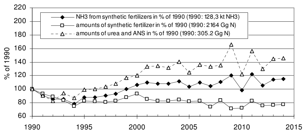
Figure 2.12: Application of mineral fertilizer N (amounts sold), amounts of N in urea and ANS applied, and the NH 3 emissions from the total application of mineral fertilizers (Submission 2016)
