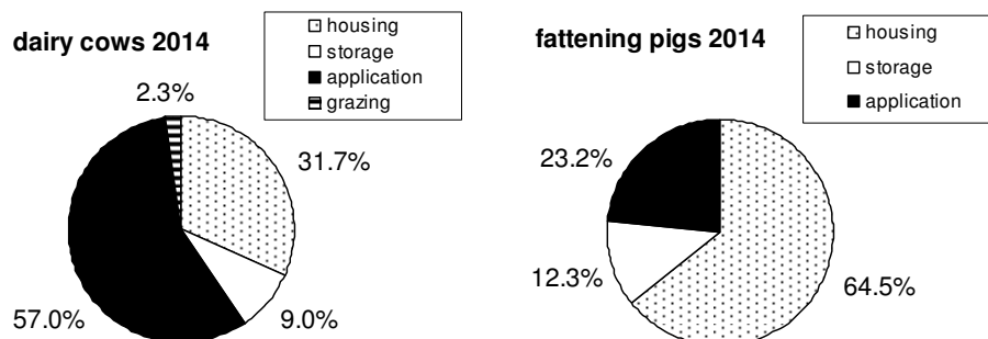
Figure 2.9: Dairy cows and fattening pigs (Submission 2016): Percentages of NH 3 emissions originating from housing, storage, manure application and grazing in 2014 (no free range husbandry for pigs)
