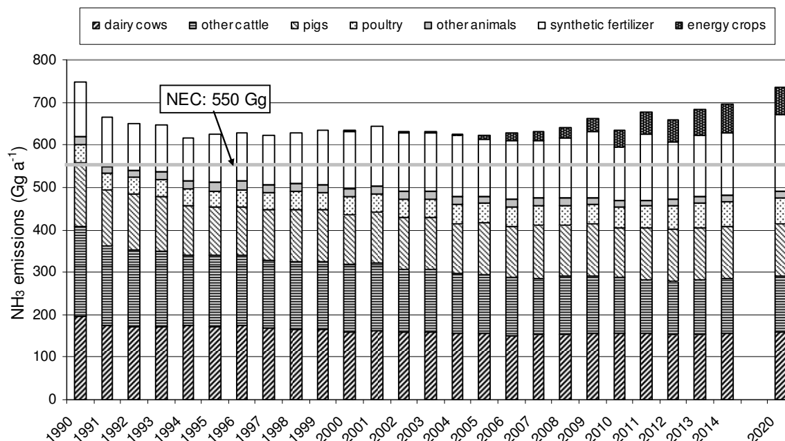
Figure 2.7: Annual NH 3 emissions from German agriculture and projections for 2020 (Submission 2016)
